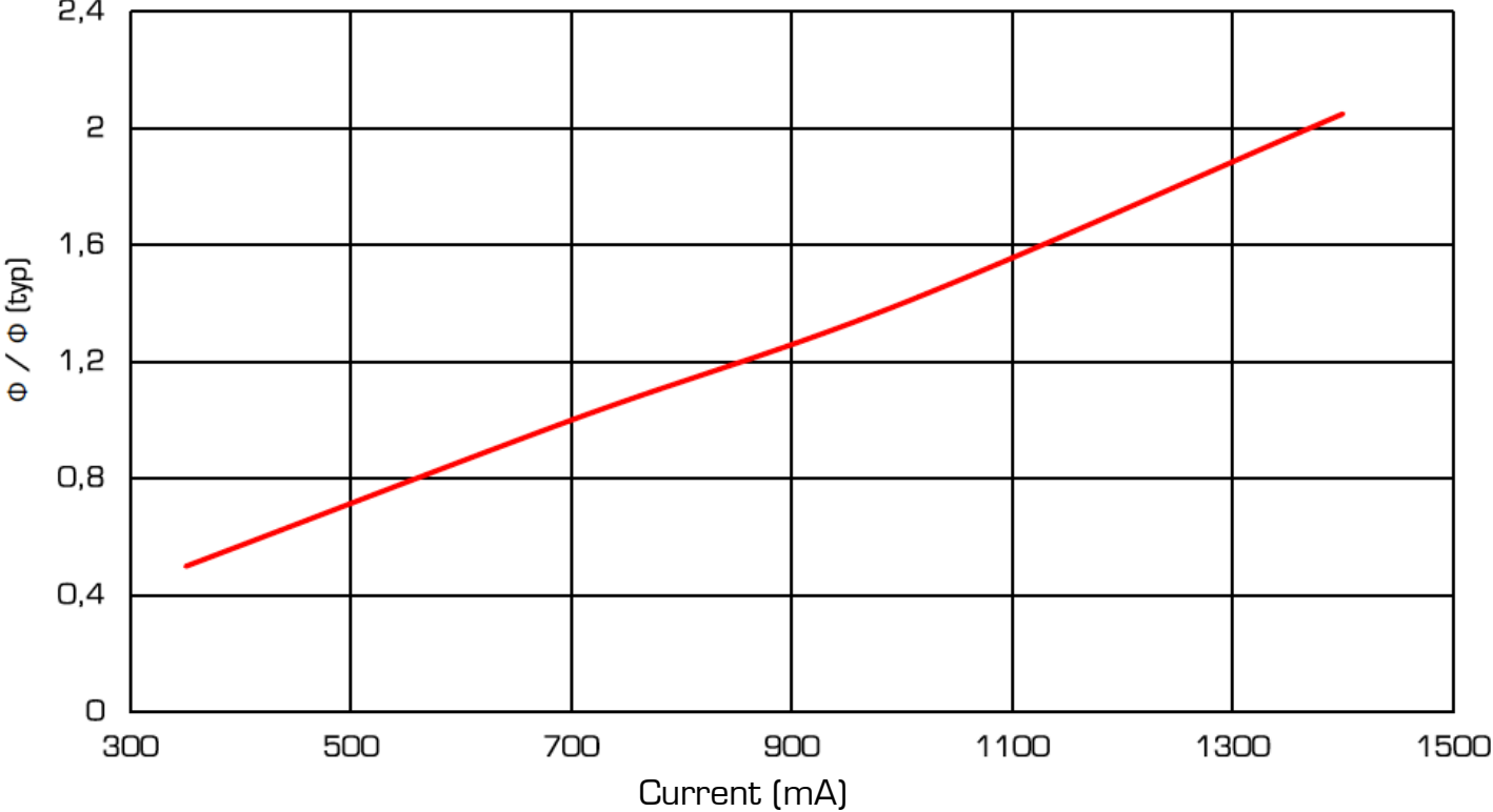
RADIANT FLUX vs. CURRENT
